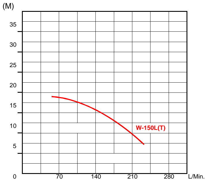
Performance Curve
